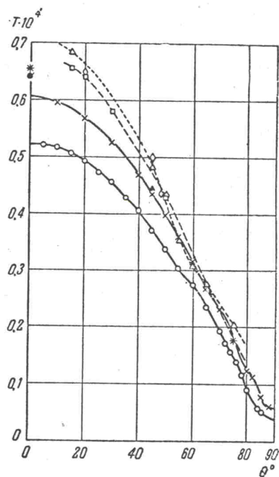
FIG. 5. Angular dependence of the oscillation period of the susceptibility caused by the smallest group of mobile charges in different zinc crystals, obtained from: x - crystal Zn-1, o - crystals Zn-2, 3, 4, 7 (this paper); \Delta - Sidoriak and Robinson, 14 \Delta - Mackinon, 19 \bullet - Berlincourt and Steele, 20 \square - Donahoe and Mix, 21 * - Dhillon and Shoenberg. 22
